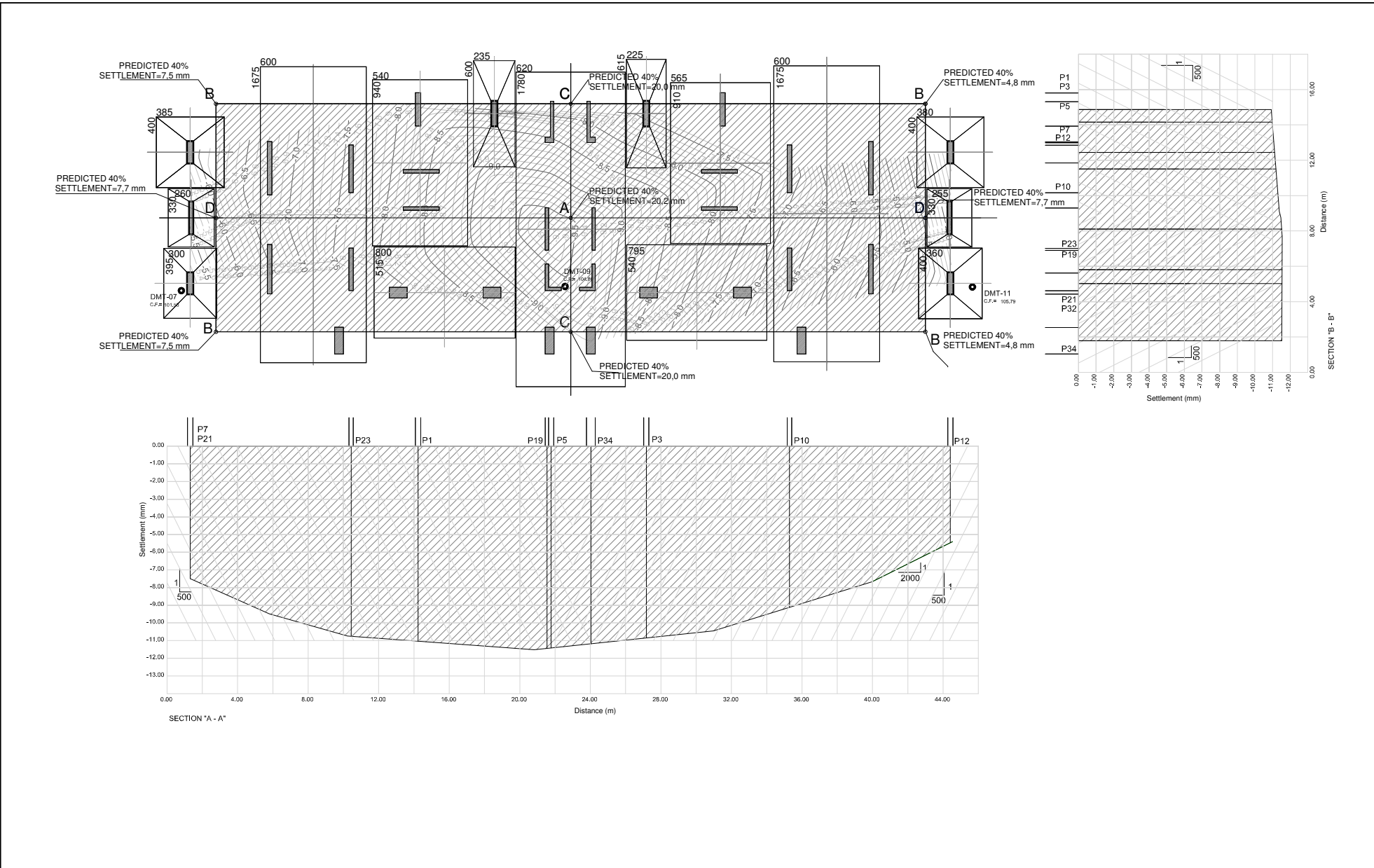
Figure 5. " Morumbi building" in construction, with 40% of the total load
